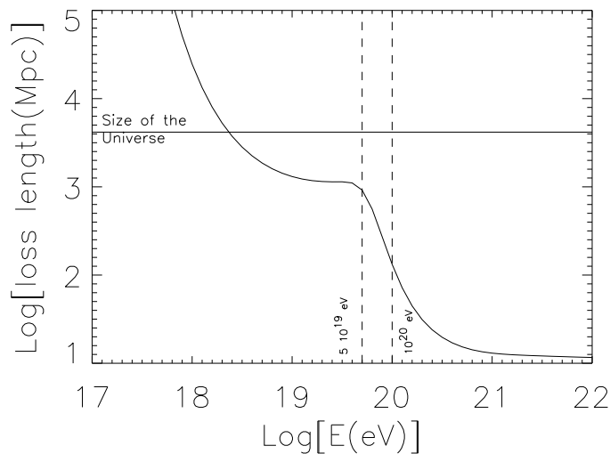
Figure 1. Loss length of UHECRs for proton pair production and photopion production.
